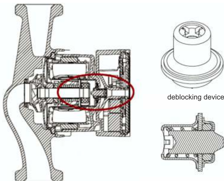
sectional drawing of deblocking device
