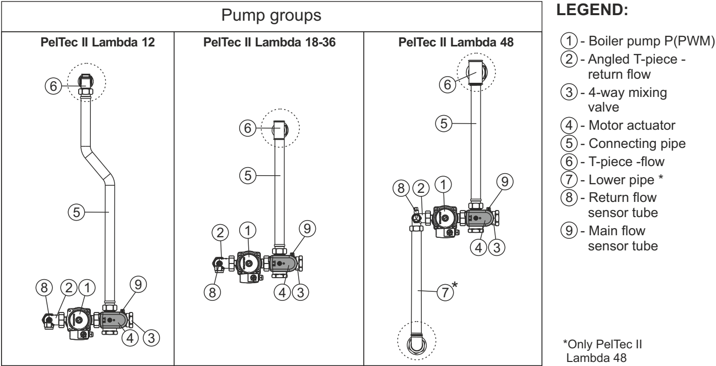
Example of installation pump group to the boiler PelTec II Lambda 18-36
