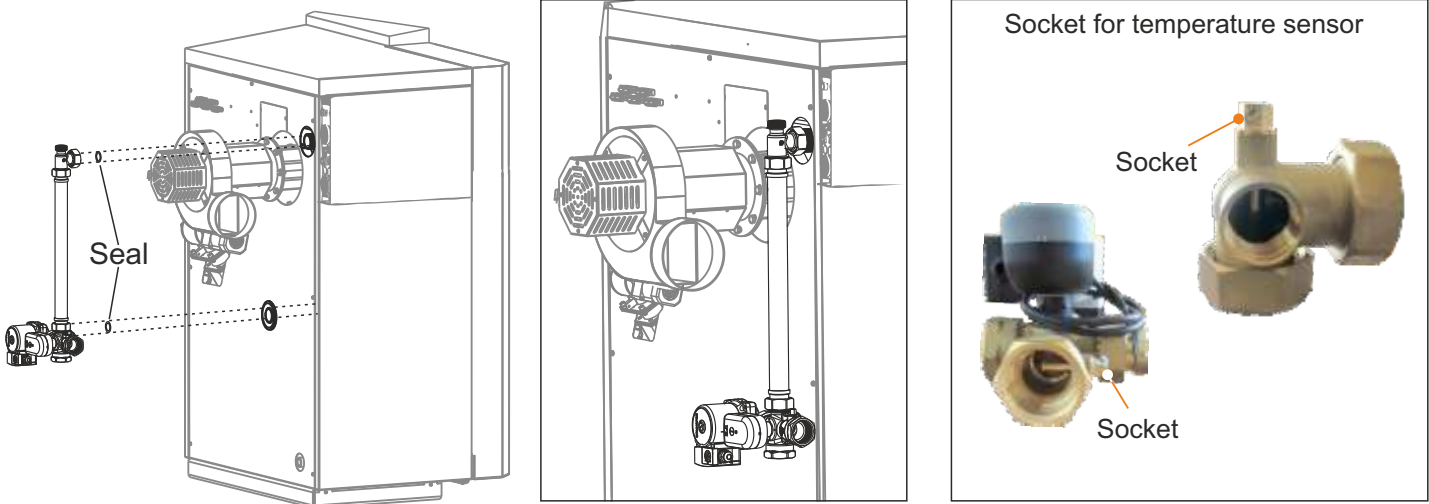
Example of installation pump group to the boiler PelTec II Lambda 18-36
